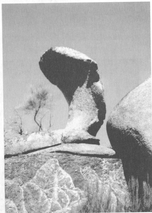
7. kép: Túlfejlődött tafoni a Boivão melletti „Castelo da Furna”-ban Picture 7.: Overdeveloped tafoni in the „Castelo da Furna” near the village of Boivão
