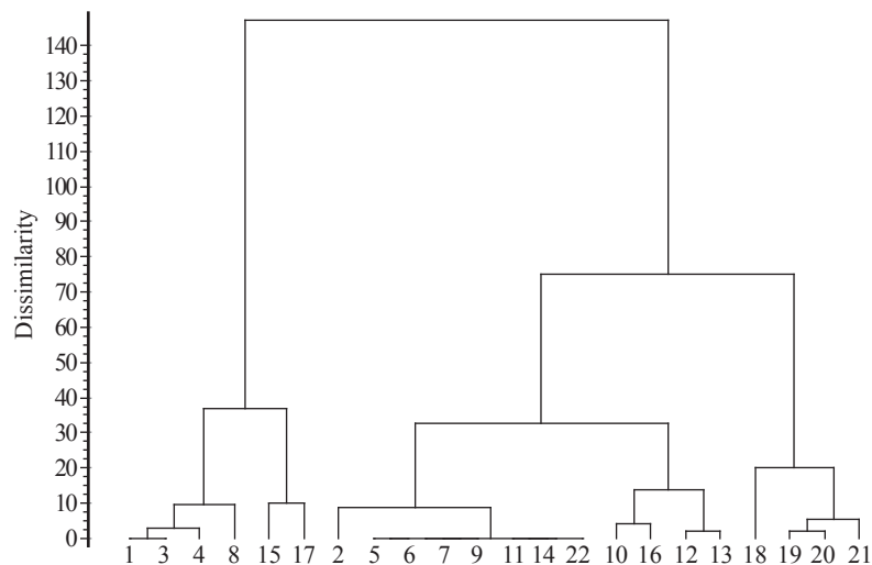
Fig. 3 Cluster analysis for Hungarian caves based on their troglotrophic Collembola species. (For location and name of the caves, see Fig. 1 and Tab. 1 respectively).
