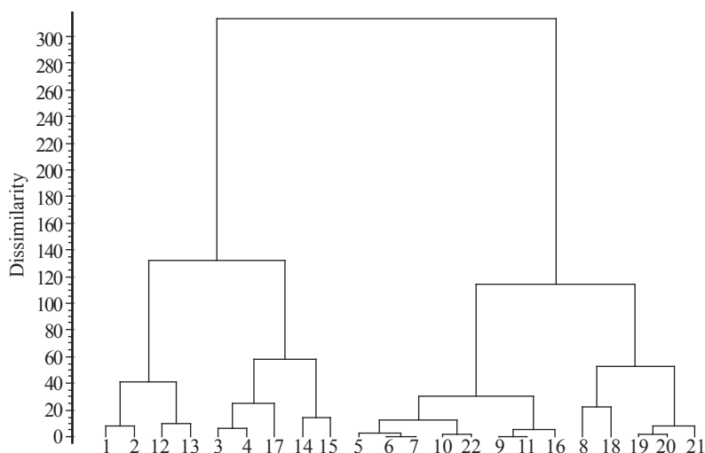
Fig. 2 Cluster analysis for Hungarian caves based on their troglotrophic and eutroglophile Collembola species. (For location and name of the caves, see Fig. 1 and Tab. 1 respectively).
